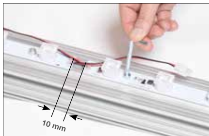
5 Add more LED-bars and connect with that before, approx 10 mm from the first one.
