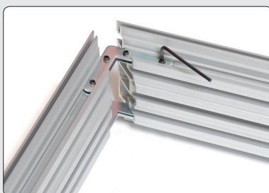
Corner connection.
