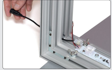
3 Insert the adaptor cable in the hole in the profile. Each hole fits 2 cables.
